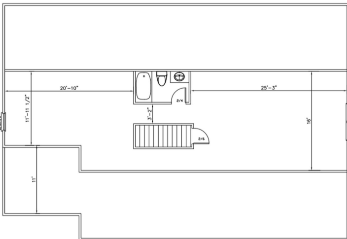
THIRD FLOOR OPTION
