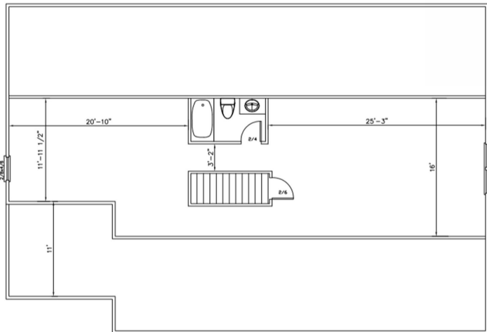
THIRD FLOOR
